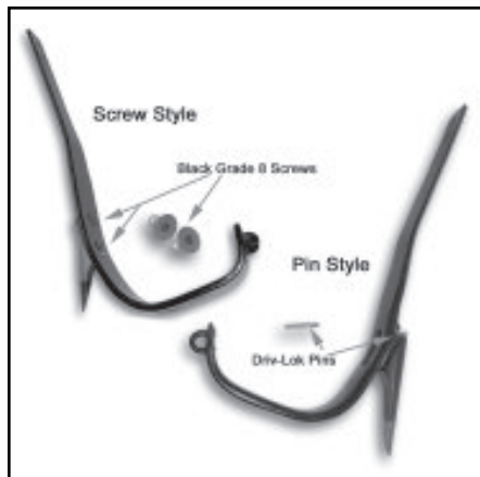
New screw type replaceable gaff.
