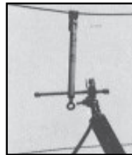
Position one end of jumper on hanger bar.
